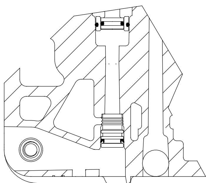
RECESSED (#1) (NON-LOCKING)
