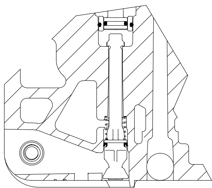
SHOWN WITH VALVE (A) & BLANK PLUG (B), BOTTOM PORTS & RECESSED WITH LEVER NON-LOCKING (#5) MANUAL OPERATOR (SEE BELOW FOR ADDITIONAL OPTIONS)
